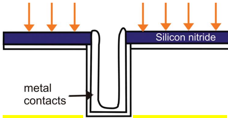
Conventional buried contact cell
